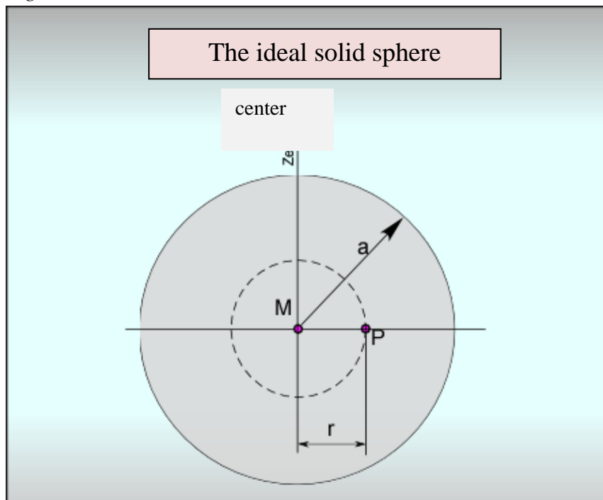
Gravity calculation for a point P inside of a solid sphere
