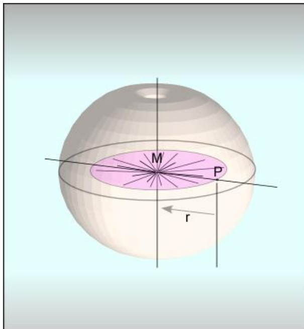
Center-oriented integral
